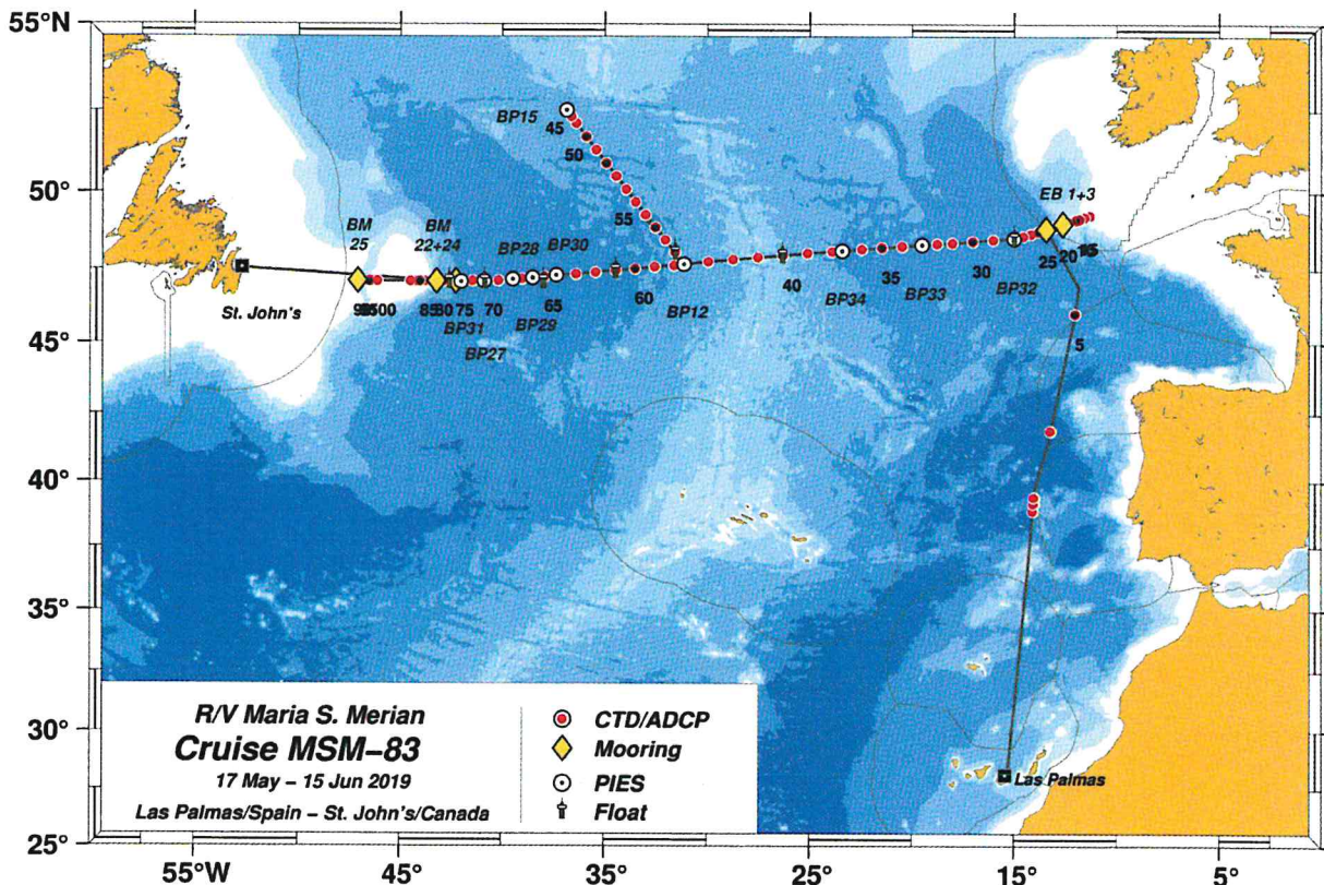
Figure 1. Track of RV MARIA S. MERIAN, cruise MSM83, and locations of hydrographic profiles (red dots denote profile dots), deployed moorings (yellow diamonds), locations of inverted echo-sounders with pressure sensors (PIES, white), and Argo float deployments. Bathymetric contours are shown every 1000 m.
